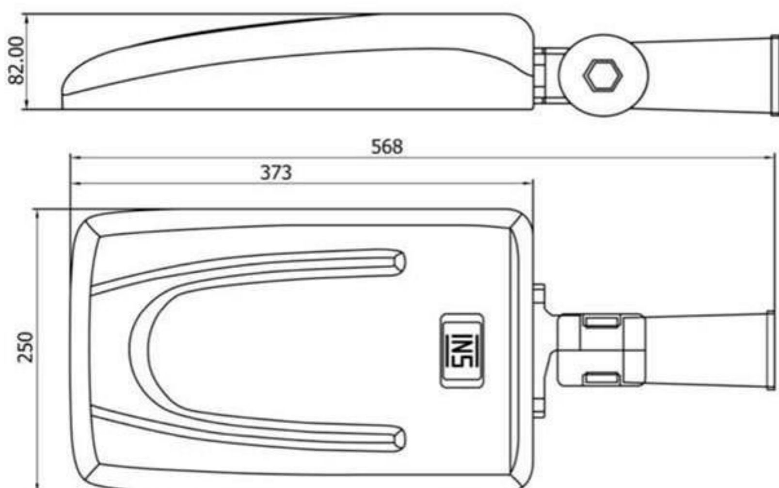
Fixture Dimension
